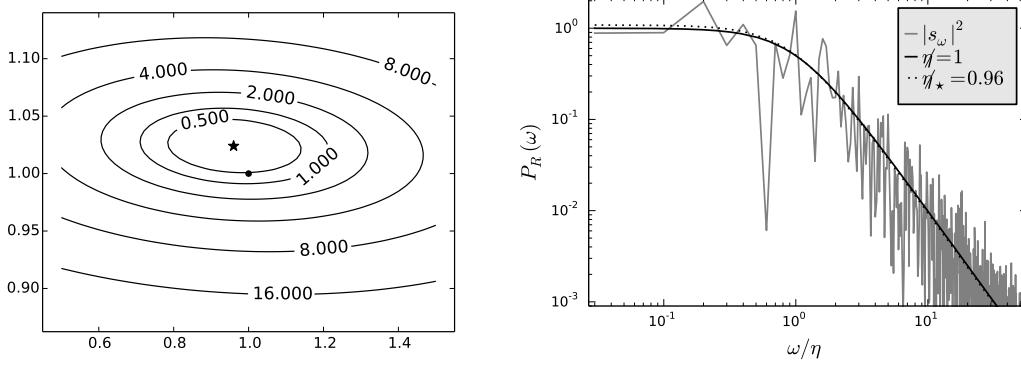
Figure 10: Parameter determination for the Ornstein-Uhlenbeck process. Left: Information Hamiltonian contours \Delta\mathcal{H}(s, a) = \mathcal{H}(s, a) - \mathcal{H}(s, a_*) as a function of (\eta, a_1) where a_0 = \eta = 2\pi\eta for the signal realization shown in Fig. 8. The minimum at (\eta, a_1)_* \approx (0.96, 1.024) is marked by a star and the correct values at (\eta, a_1) = (1, 1) by a dot. The correct value lies on the so called 1- \sigma contour at \Delta\mathcal{H} = 1/2 . Right: Power spectrum of the signal realization shown in Fig. 8, that of the original process, and that for the reconstructed parameters a_* .
