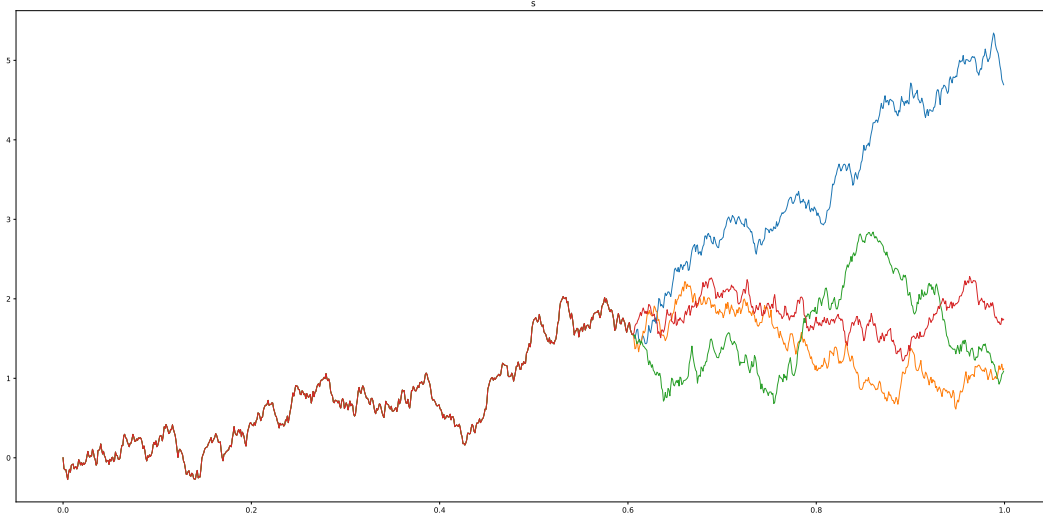
Figure 7: Evolution of a stock prize signal, which is known up to the present time t (red line), and afterwards being unknown. The uncertainty standard deviation \sqrt{D_{(t)}^{ff}} grows with the future time f as \propto \sqrt{f-t} in case of a constant volatility \sigma .
