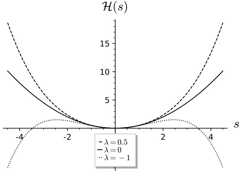
Figure 11: \mathcal{H}(s) = \frac{1}{2}s^2 + \frac{\lambda}{4!}s^4 for three values of \lambda , illustrating that next below \lambda = 0 the information Hamiltonian becomes unbound from below and consequently the partition function diverges. This is the reason why the expansion has a convergence radius of zero and is only an asymptotic expansion.
